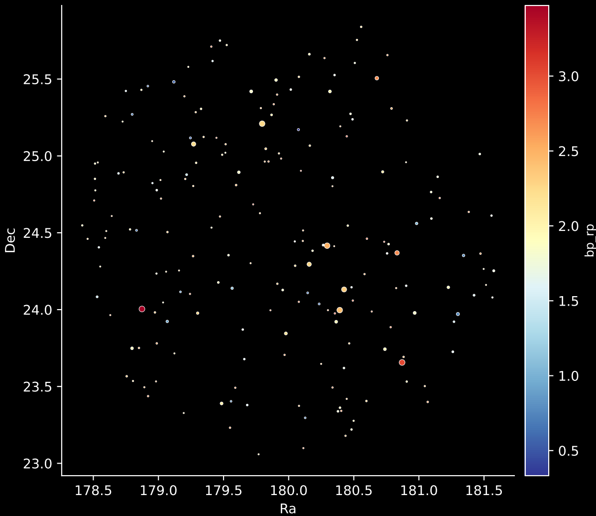
APOGEE DR17 Field: [SGRT-1] Stars: 202
