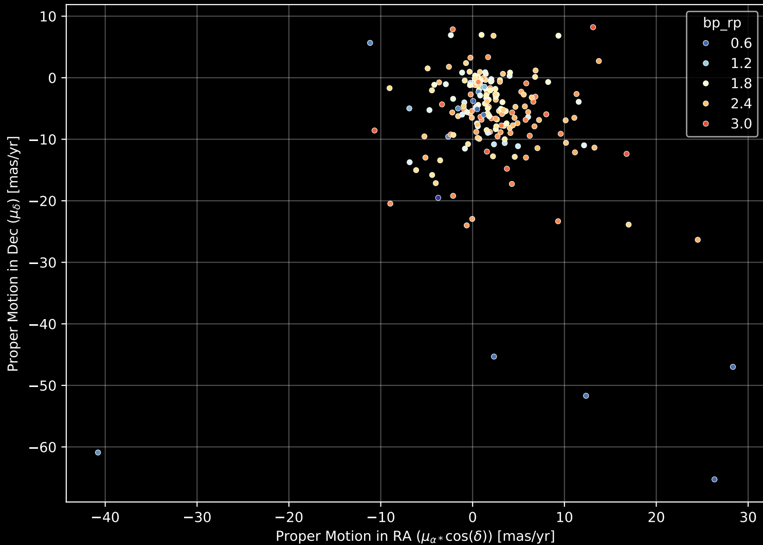
APOGEE DR17 Field: [SGRT-1] Proper Motion Diagram (n= 202)
