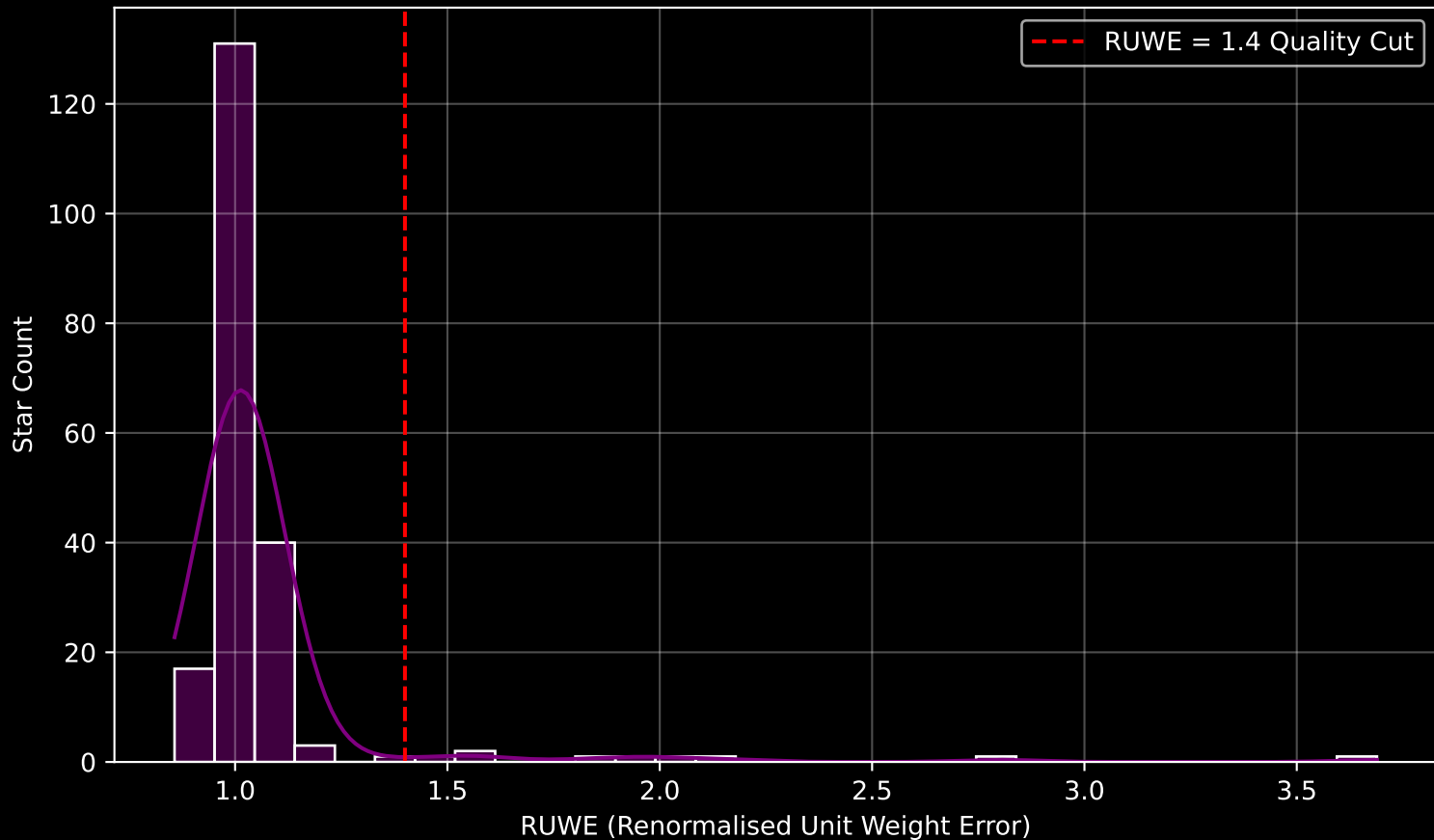
GAPOGEE DR17 Field [SGRT-1] RUWE Distribution (n= 201)
