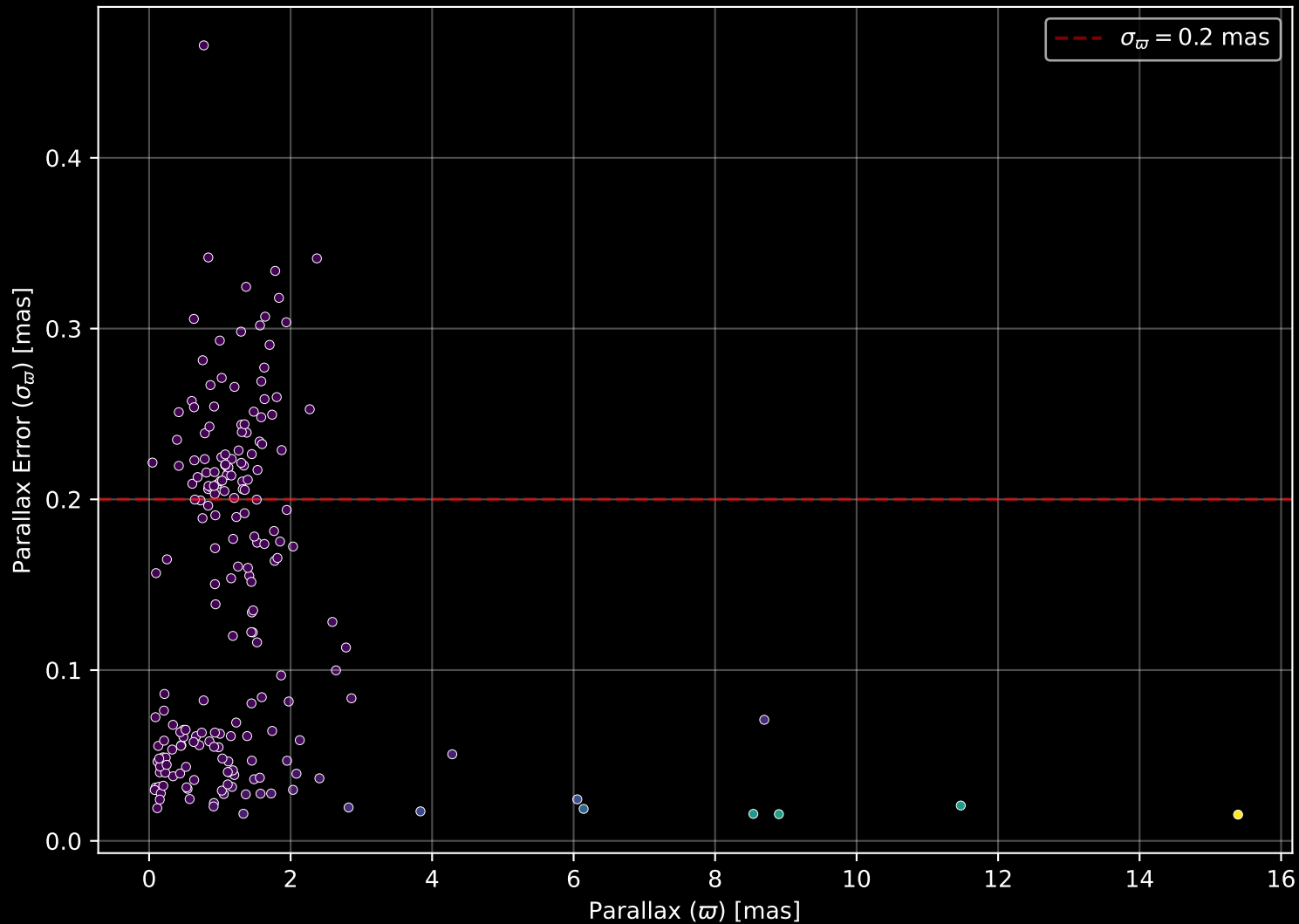
APOGEE DR17 Field: [SGRT-1] Parallax Quality (n= 202)
