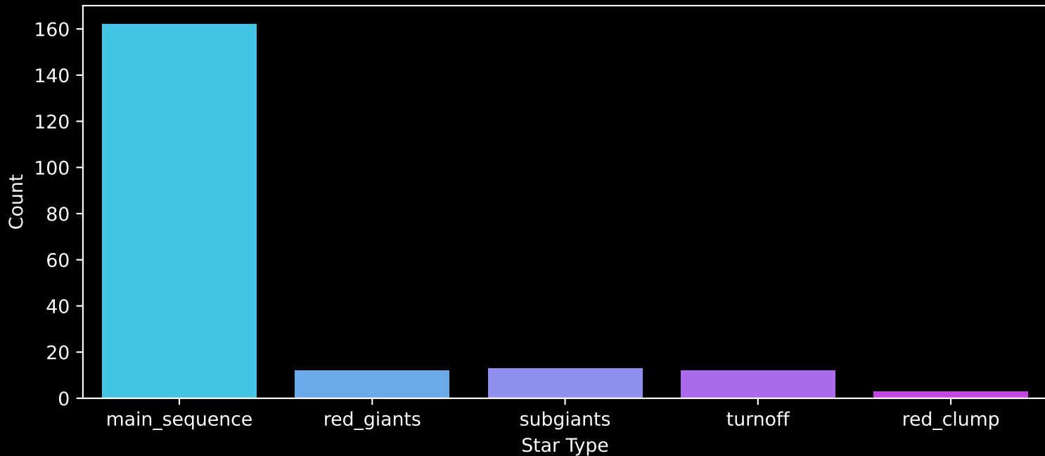
APOGEE DR17 Field: [SGRT-1] Count plot of Star Type
