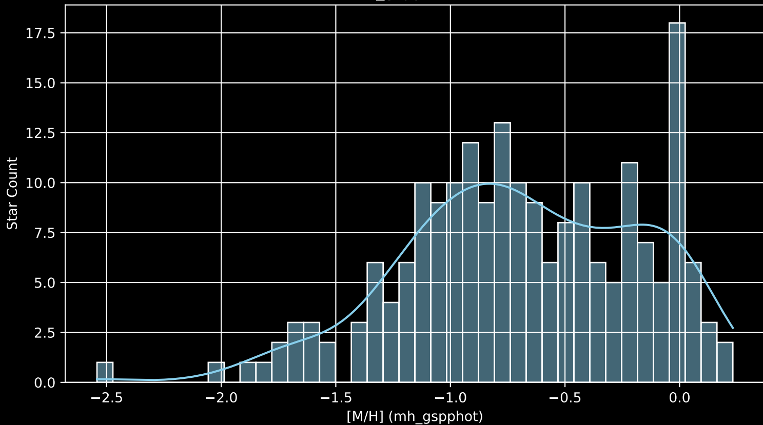
APOGEE DR17 Field: [SGRT-1 [M/H] (mh_gspphot) (n= 202)
